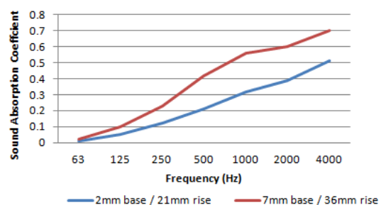
Profiled Absorption Coefficients: BS EN 20354 (Reverberation Room)
